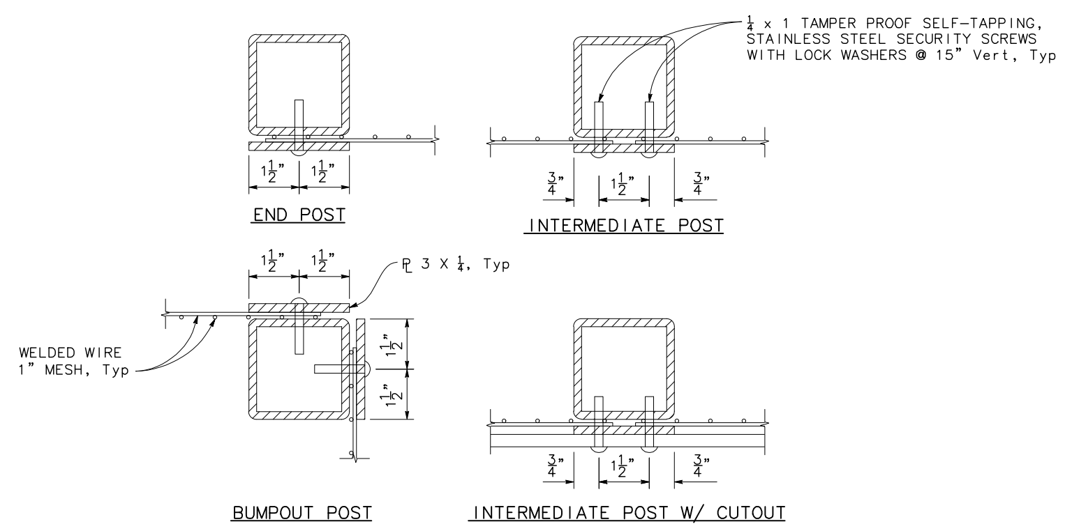
TYPICAL POST SECTIONS (TYPE B) NO SCALE
