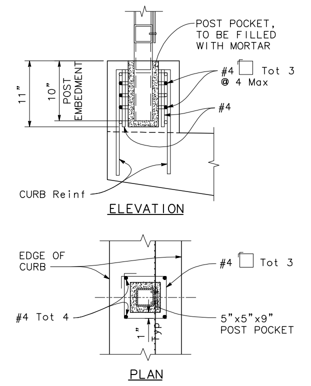
RAILING ANCHORAGE DETAILS (TYPE B) 1 1/2"=1'-0"
