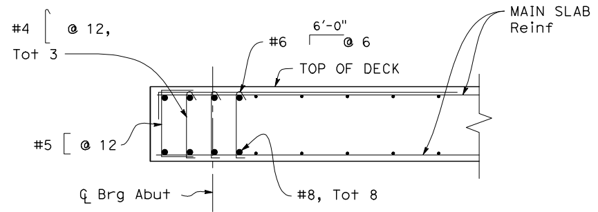
END DIAPHRAGM 3/4" = 1'-0"
