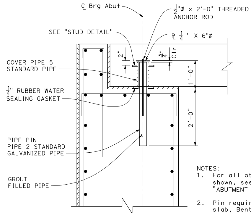
PIPE PIN DETAIL 1" = 1'-0"
