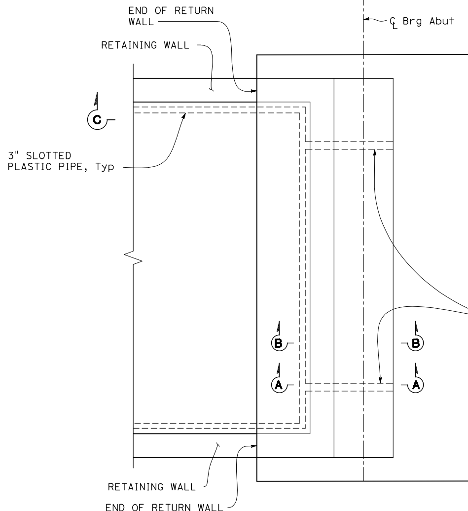
PLAN 1/2"=1'-0"
