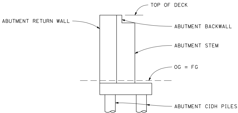
STEP 1
