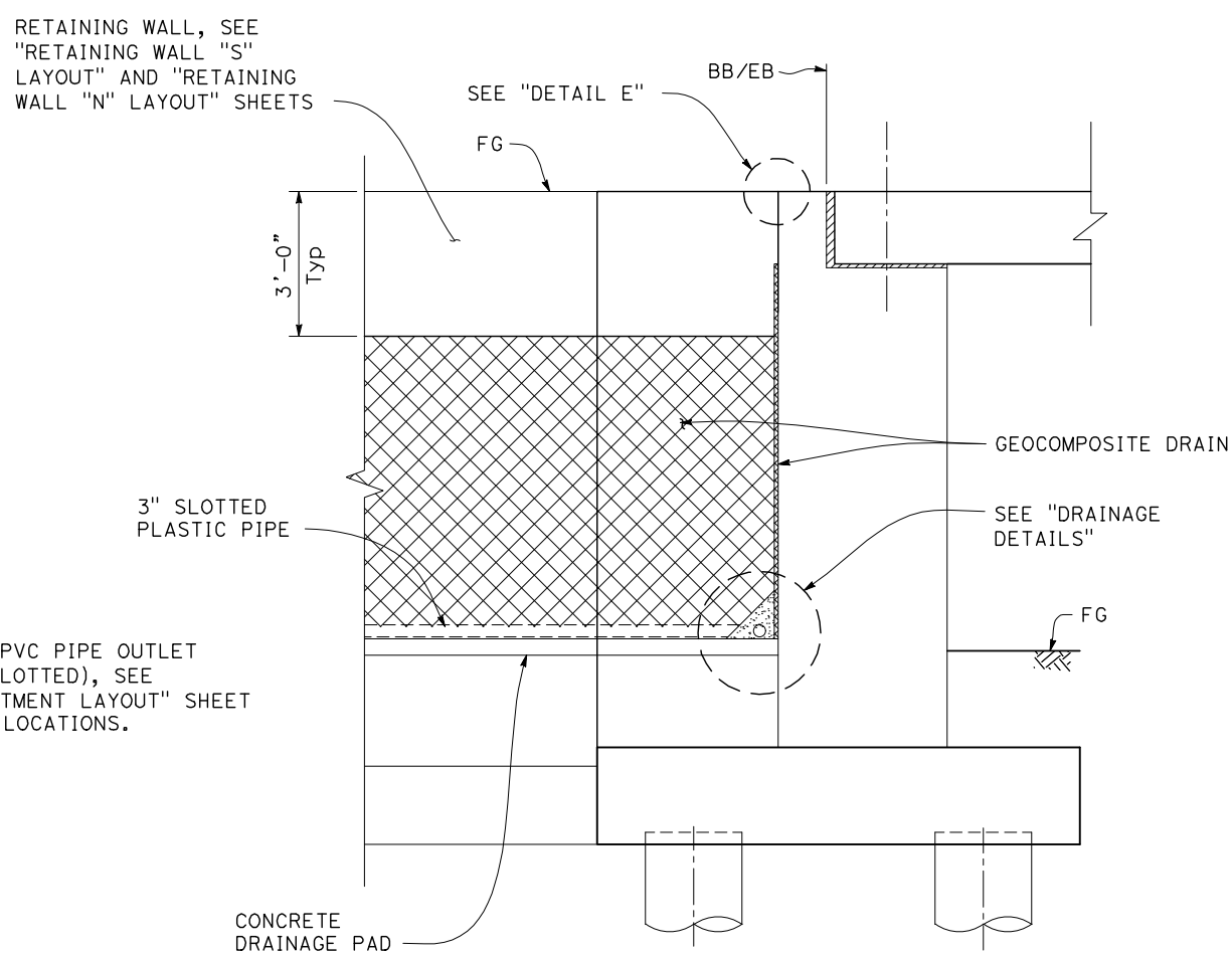
SECTION C-C 1/2" = 1'-0"
