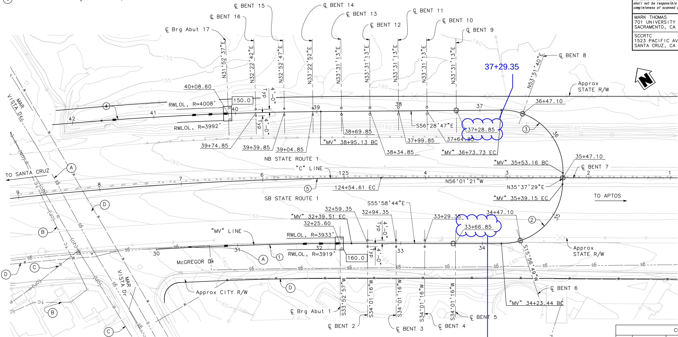
PLAN 1" = 30'
