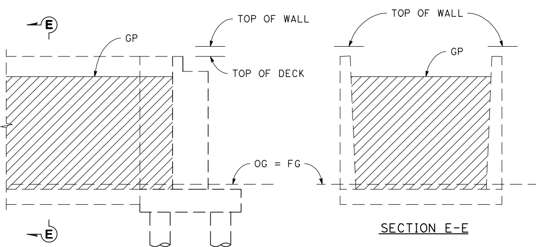
STEP 3 AND 4
