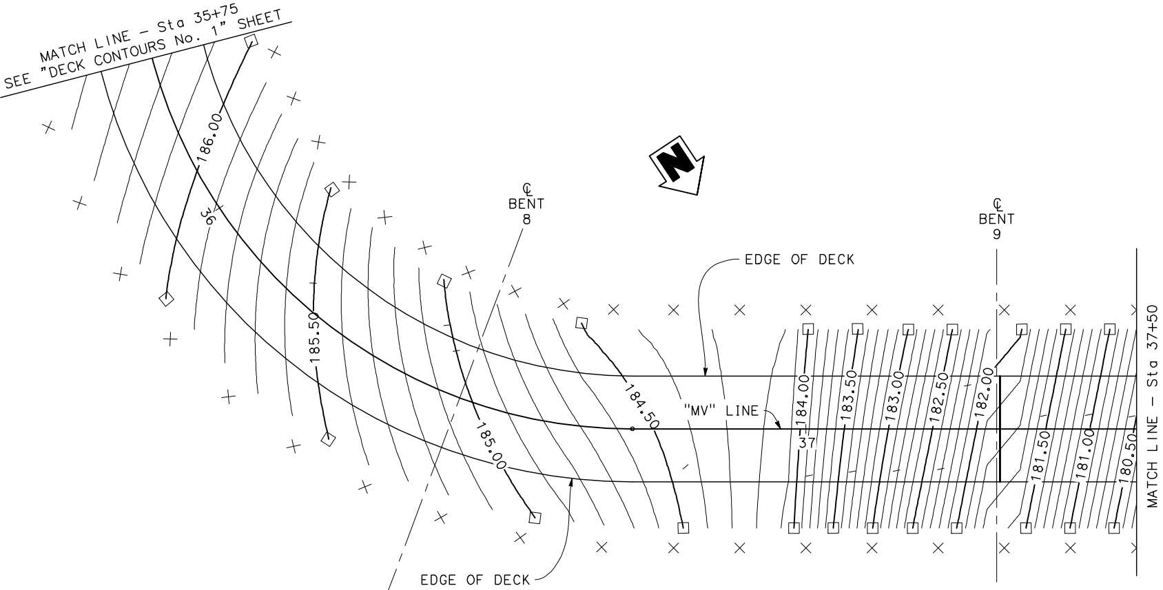
PLAN 1" = 10'
