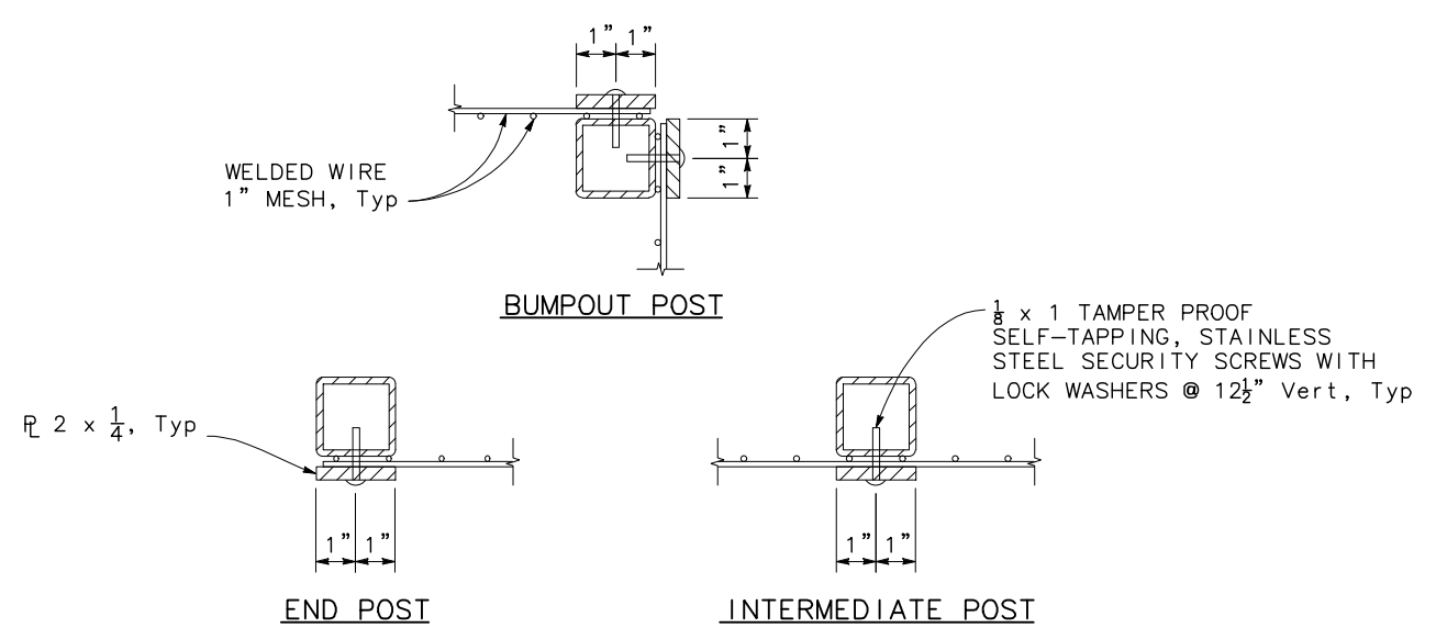
TYPICAL POST SECTIONS (TYPE A) NO SCALE
