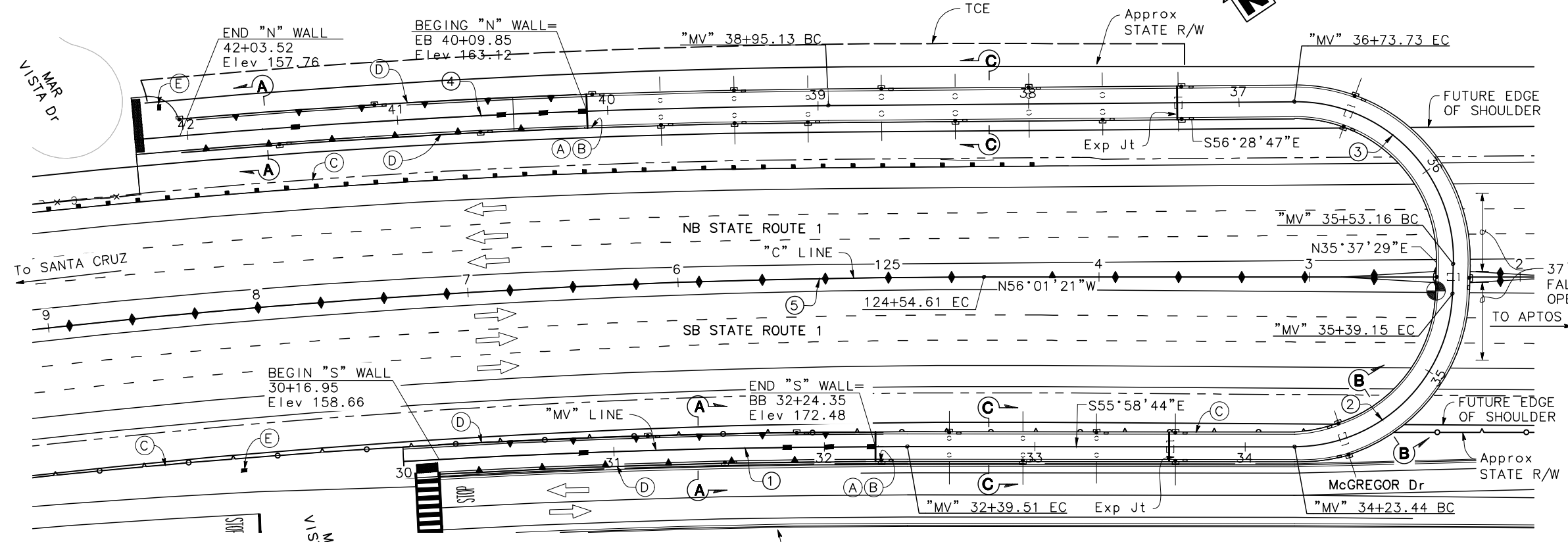
PLAN 1" = 30'
