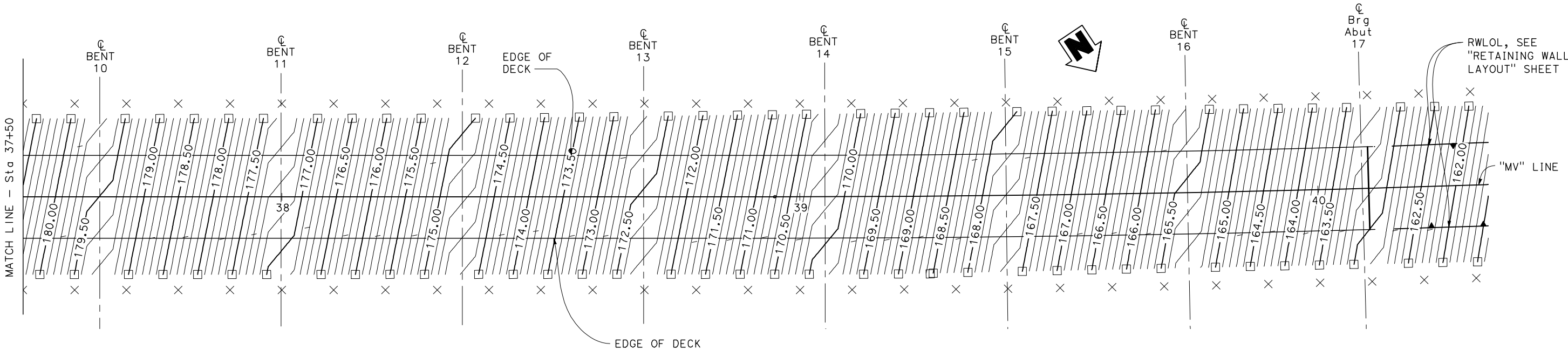
PLAN 1" = 10'
