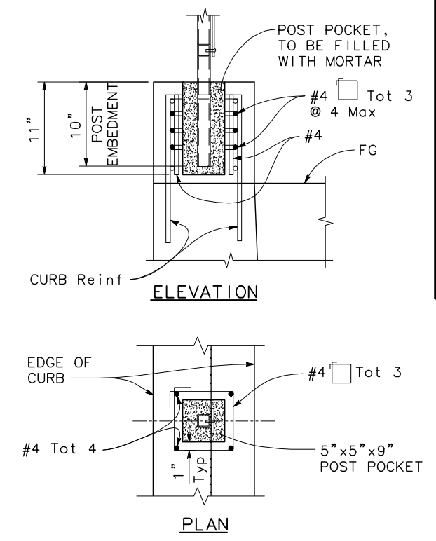
RAILING ANCHORAGE DETAILS (TYPE A) 1 1/2"=1'-0"
