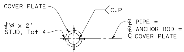
STUD DETAIL 1" = 1'-0"
