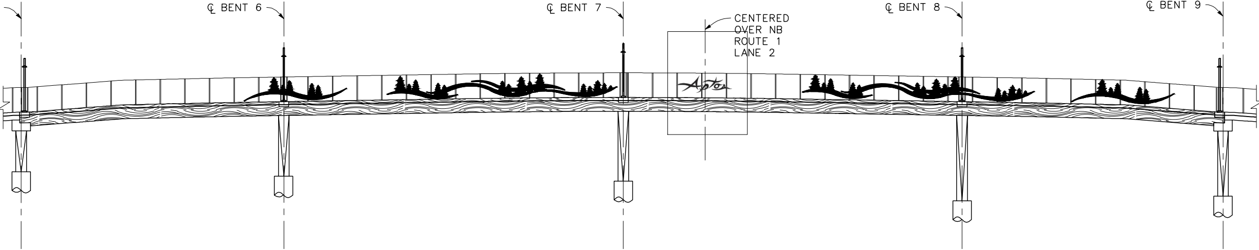
ELEVATION - NB FACING RAILING NO SCALE
