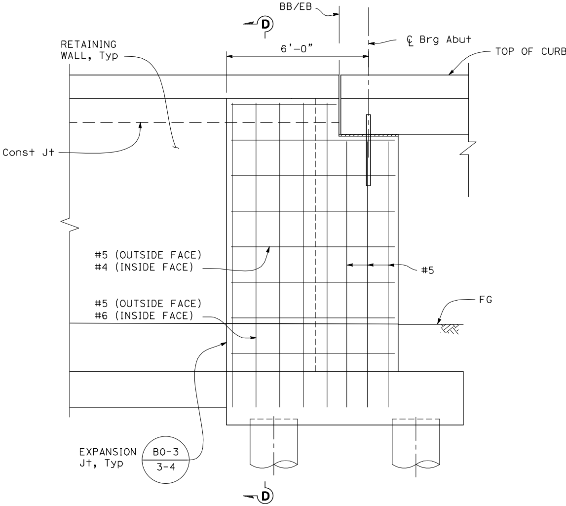
RETURN WALL ELEVATION
