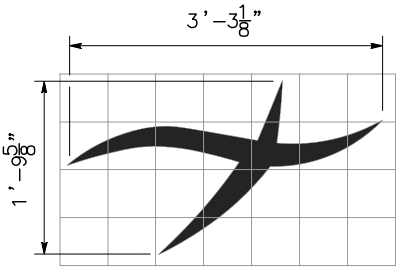
CUTOUT "E" 1/2" = 1'-0"
