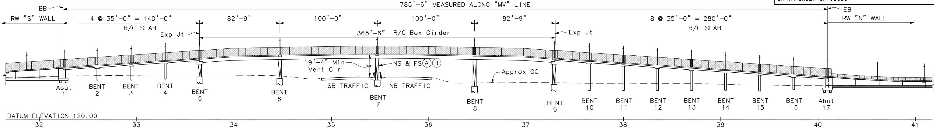
DEVELOPED ELEVATION 1" = 30'
